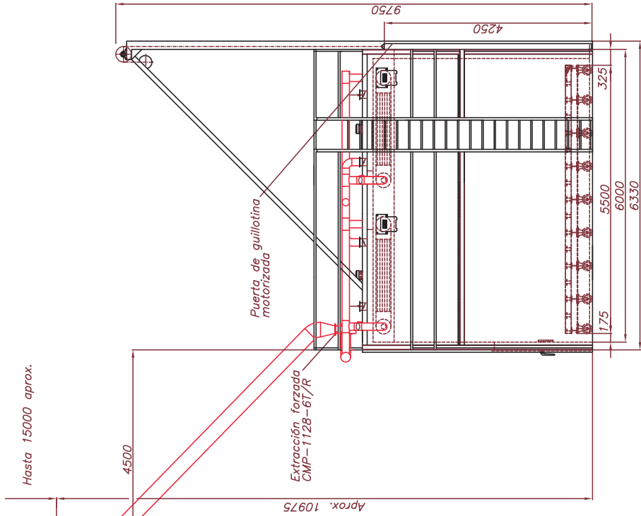
LATERAL
